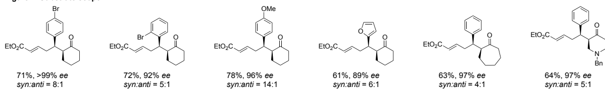
Figure 1. Substrate scope
