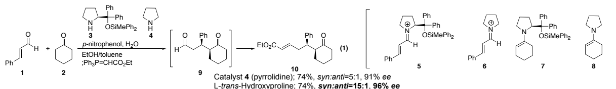
Figure 1. Substrate scope
