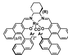
Ru-salen 1: Ar = 2,6-F 2 C 6 H 3
