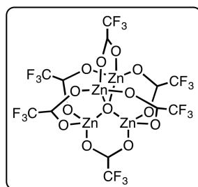
Zinc cluster (1)
